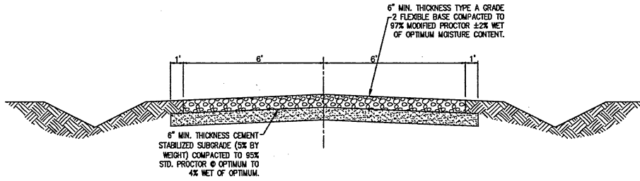
ROAD DETAIL NOT TO SCALE
