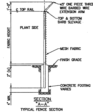
SECTION "A-A" TYPICAL FENCE SECTION
